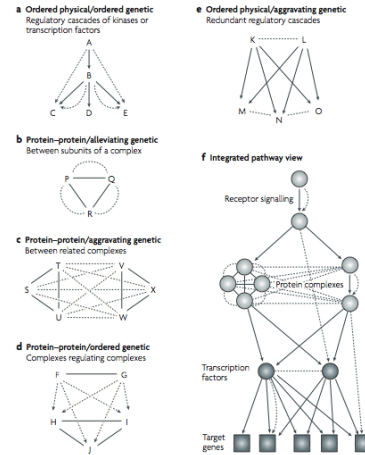
Figure 4 | Network motifs assembled from different combinations of interaction measurements. Physical interactions are shown as solid lines and arrows, and genetic interactions are shown as dashed lines and arrows. Part a shows an example of integrating ordered physical versus ordered genetic interactions, in which knockout of A or B results in changes in the activity of C, D and E (ordered genetic interactions), which are brought about because of changes in transcriptional activity or kinase-substrate binding (ordered physical interactions) 13,14,18,19 . Members of protein complexes (protein-protein interactions) can be connected by genetic interactions either within complexes (shown in part b) or between complexes (shown in part c) 17,19,20,21 . In part d, members of a complex made up of F-G (protein-protein interactions) operate upstream of or epistatically to (ordered genetic) the complex H-I-J 22 . In part e, regulatory factors K and L cooperate to activate targets M, N and O (ordered physical) which function in parallel pathways (alleviating genetic) 23,24 . Part f shows how the motifs of previous panels might combine within a still larger network, starting at a receptor protein and ending at transcription factors modulating the expression of target genes. Note that the motifs in each panel are summarized from the literature (see references provided) and are not intended as an exhaustive catalogue of all ways of integrating interactions.
